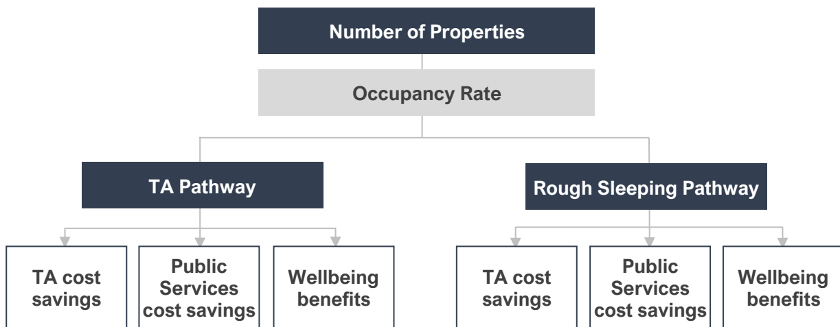
Figure 2. High-level methodology
